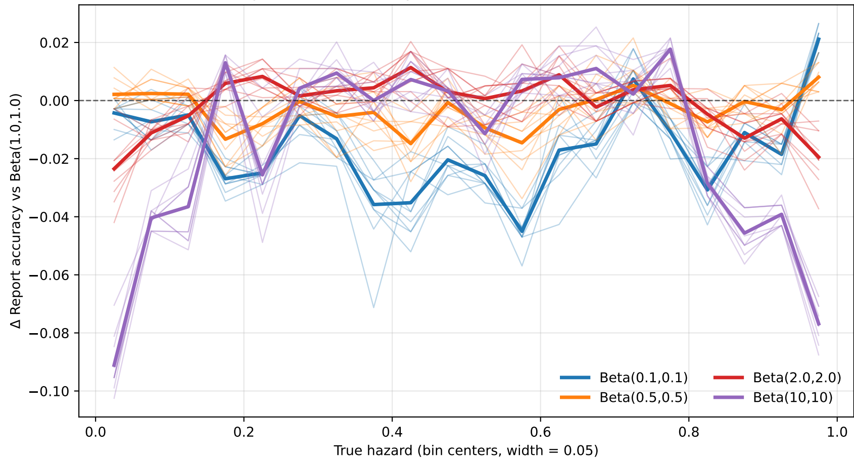
Report-head: accuracy difference relative to Beta(1.0,1.0)
